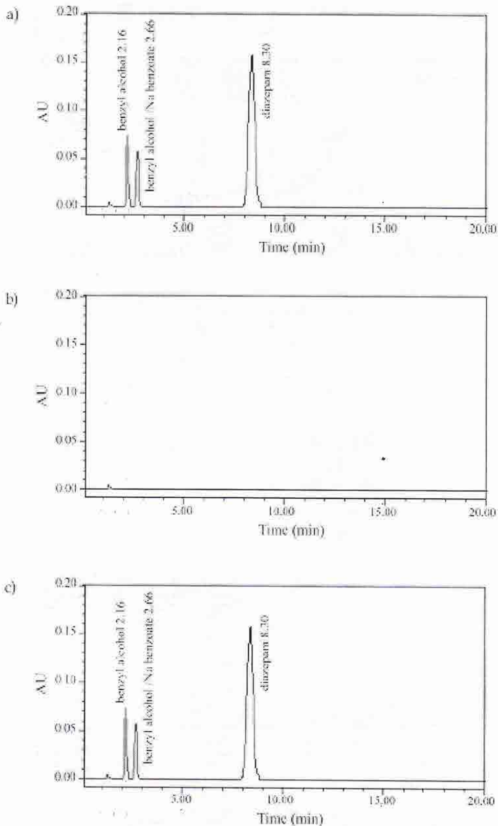
Fig. 1. Chromatograms of: a) standard solution of DZP ( 0.05 \text{ mg mL}^{-1} ), benzyl alcohol ( 0.375 \text{ } \mu\text{g mL}^{-1} ), benzoic acid ( 0.025 \text{ } \mu\text{g mL}^{-1} ) and sodium benzoate ( 0.05 \text{ } \mu\text{g mL}^{-1} ); b) blank solution without DZP, benzyl alcohol, benzoic acid and sodium benzoate, and c) sample solution of DZP ( 0.05 \text{ mg mL}^{-1} ), benzyl alcohol ( 0.375 \text{ } \mu\text{g mL}^{-1} ), benzoic acid ( 0.025 \text{ } \mu\text{g mL}^{-1} ) and sodium benzoate ( 0.05 \text{ } \mu\text{g mL}^{-1} ).
