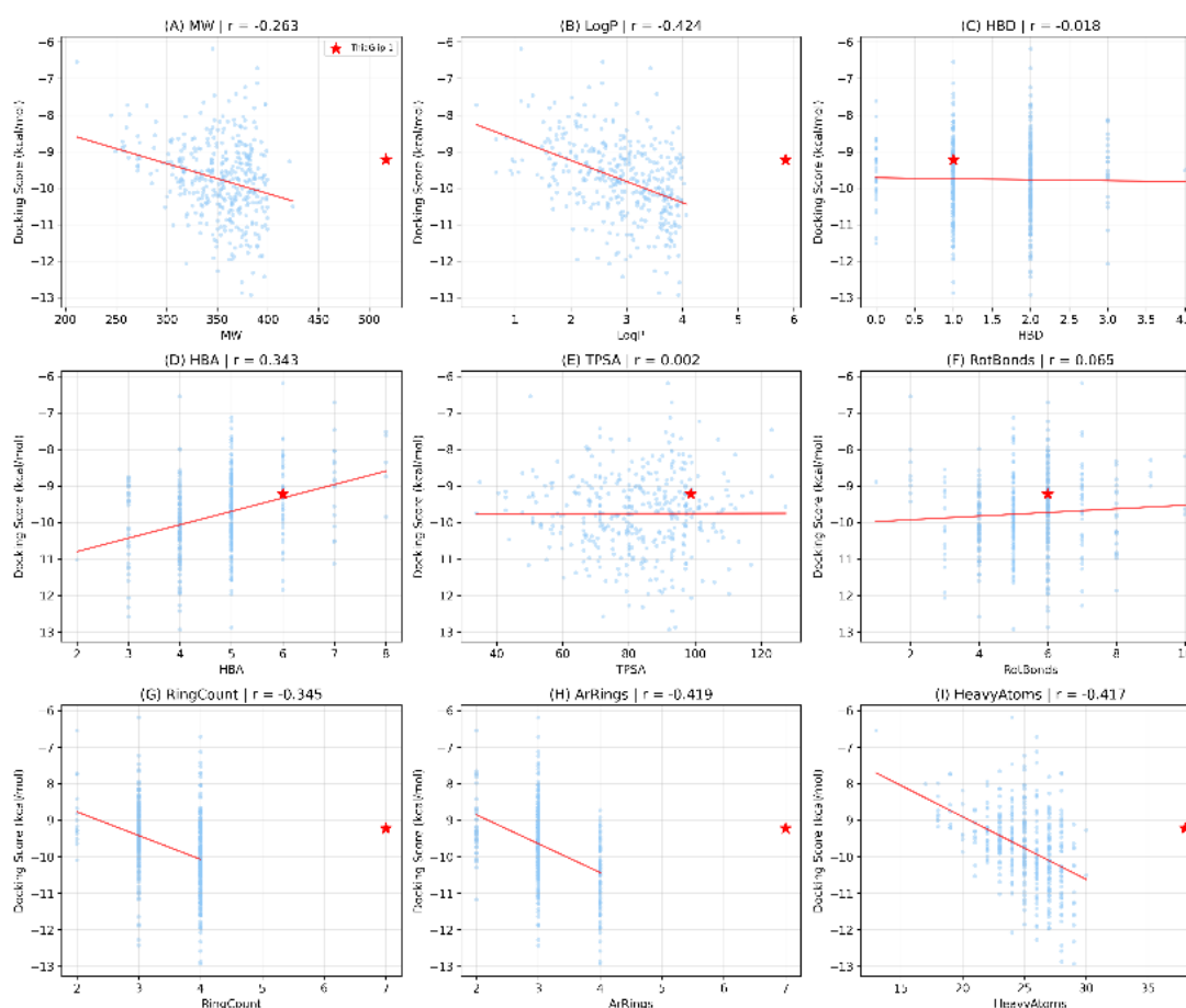
Figure (4): SAR evaluation of the virtual library of 380 compounds. Scatter plots display Pearson correlation coefficients among nine physicochemical descriptors (MW, LogP, HBD, HBA, TPSA, RotBonds, RingCount, ArRings, HeavyAtoms) and AutoDock Vina docking scores. The most significant moderate correlations were found for LogP ( r = -0.424 ), ArRings ( r = -0.419 ) and HeavyAtoms ( r = -0.417 ), suggesting that lipophilicity and aromatic ring content are the main physicochemical indicators of GLP-1R binding affinity in this library.
